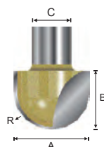
Half Round Grooving 圓底刀
