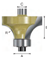
Corner Rounding with Bearing 圓角刀
