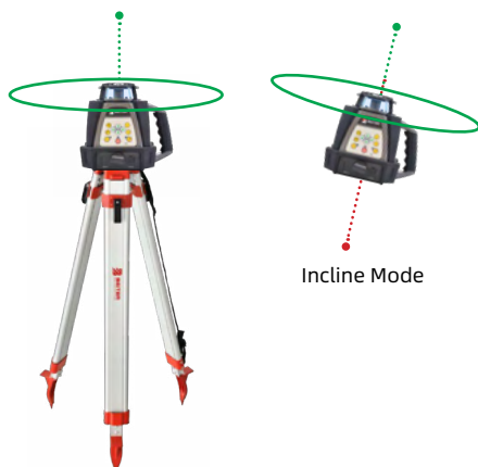
2 Plumb Dots
